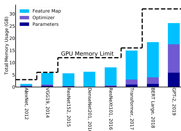
FIGURE 4. The amount of memory required to train different NN models. Here, the optimizer used for CV models is SGD+Momentum, and for NLP models it is ADAM. There is an interesting trend in discovering/designing new models, based on the available GPU memory size. Every time the GPU memory capacity is increased, data scientists have designed newer models. As such, breaking this so-called GPU memory wall could further allow new innovations. See Jain et al. 6 for more details on checkpointing.
